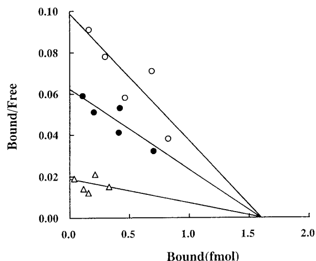
Figure 2. Scatchard plot analysis. [ 125 I]PYYP binding to SK-N-MC cells was performed in the absence (○) or presence of 10s (200 nM, ●) or 14c (50 nM, △).
